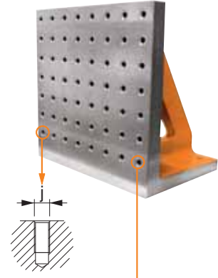
Gövdeye dişli Referans Nr. 2570 Threaded body Reference No. 2570
